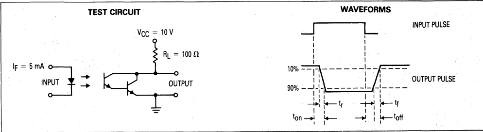
Figure 9. Switching Times
