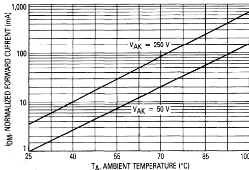
Figure 4. Forward Leakage Current versus Temperature
