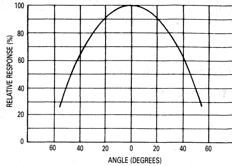
Figure 2. Angular Response
