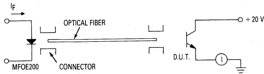
Figure 3. Responsivity Test Configuration
