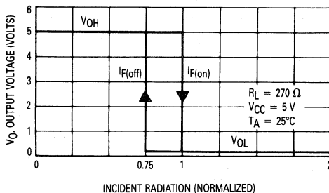
Figure 1. Transfer Characteristics
