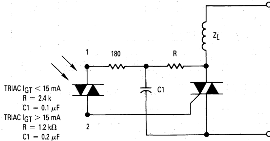
Figure 8. Inductive Load
