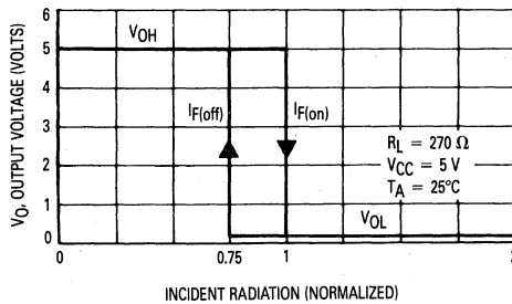
Figure 1. Transfer Characteristics
