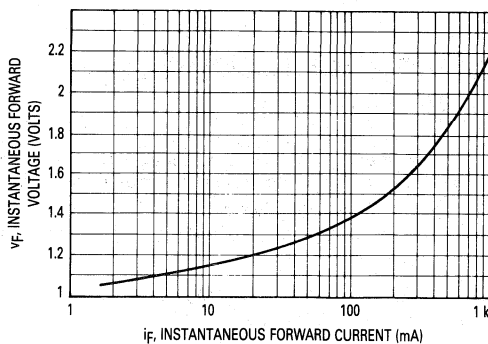
Figure 2. Forward Characteristics
