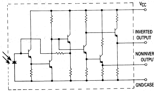
Figure 1. Equivalent Schematic
