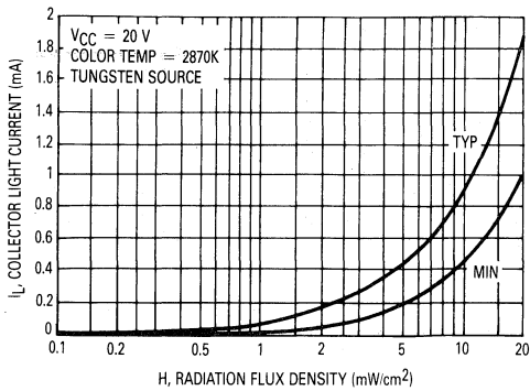
Figure 1. Collector-Emitter Sensitivity
