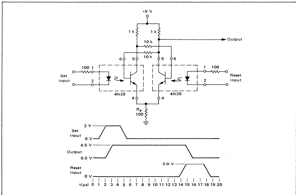
FIGURE 17 – Optically Coupled R-S Flip-Flop
