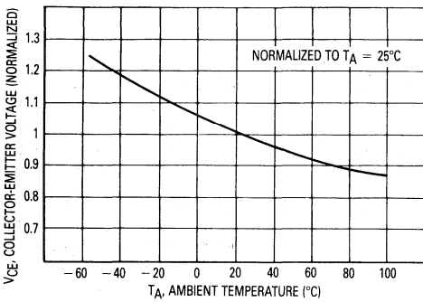
Figure 5. Collector-Emitter Voltage versus Ambient Temperature
