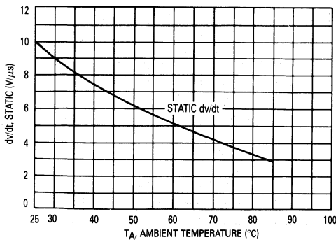
Figure 4. dv/dt versus Temperature
