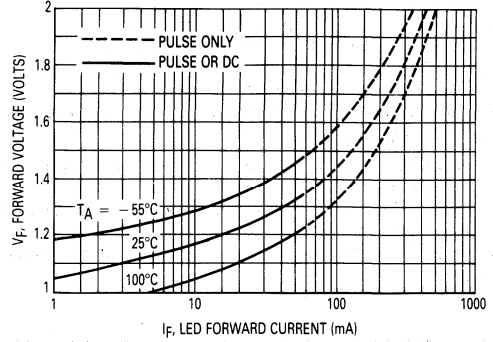
Figure 4. Forward Characteristics
