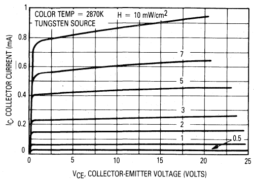
Figure 2. Collector-Emitter Characteristics
