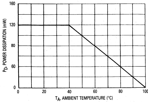
Figure 1. Power Dissipation
