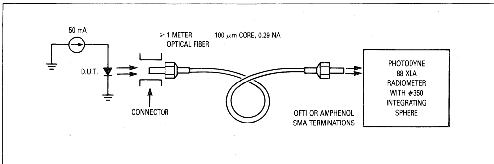
Figure 6. Coupling Efficiency
