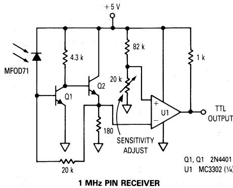
Figure 7. TTL Receiver
