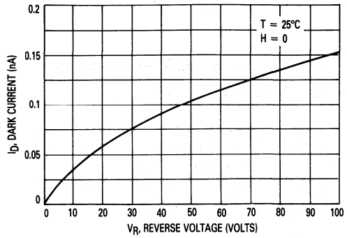
Figure 2. Dark Current versus Reverse Voltage
