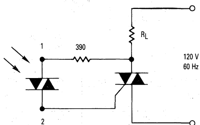
Figure 7. Resistive Load
