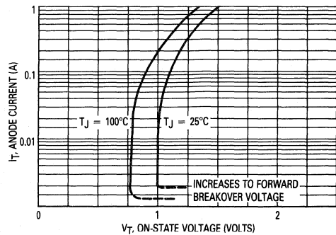
Figure 2. On-State Characteristics
