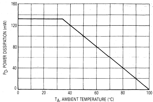
Figure 8. Power Dissipation
