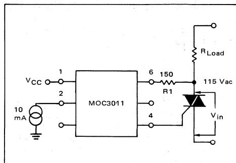
FIGURE 3 — Simple Triac Gating Circuit
