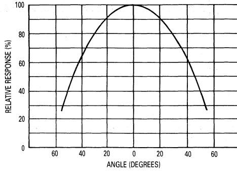
Figure 1. Angular Response
