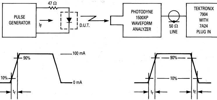
Figure 7. Rise and Fall Time Measurement Circuit
