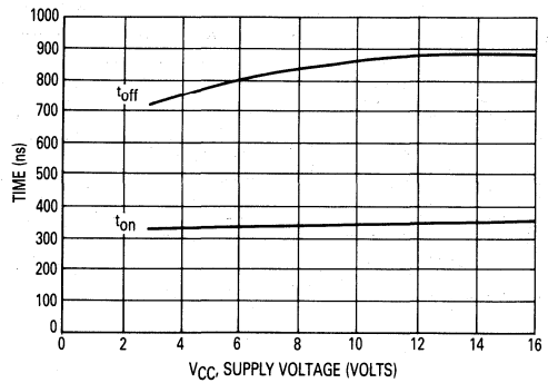
Figure 9. Total Switching Time versus Supply Voltage
