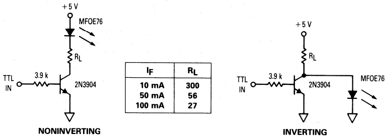
Figure 6. TTL Transmitters
