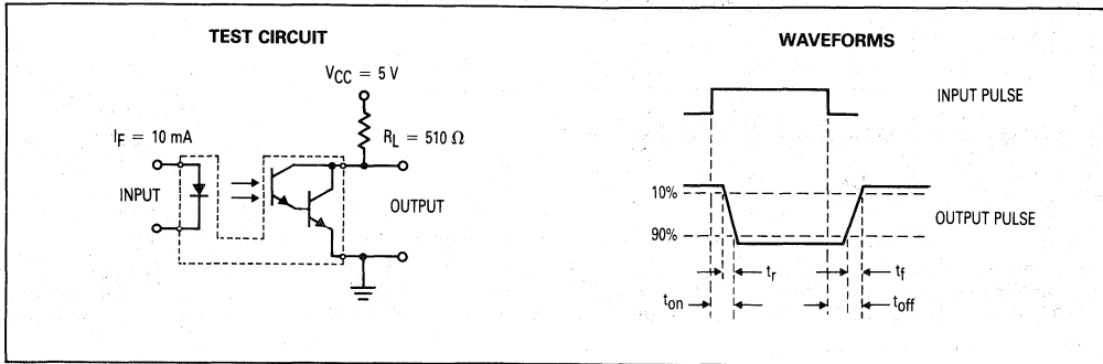
Figure 9. Switching Times
