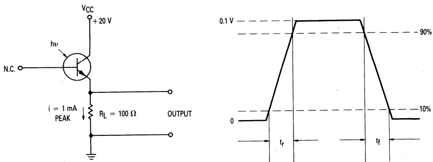
Figure 8. Pulse Response Test Circuit and Waveform
