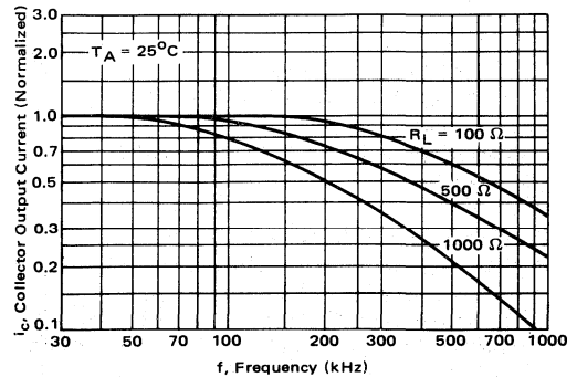
FIGURE 6 - Frequency Response
