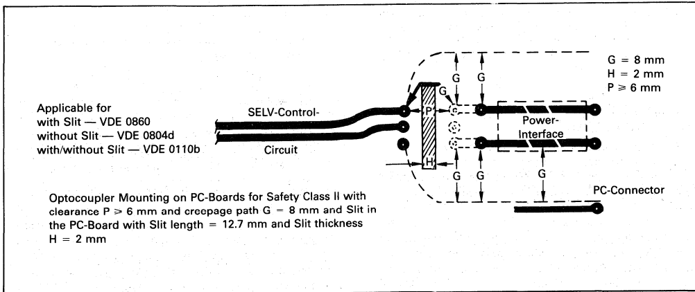
Figure 4. Optocoupler Mounting on PC Boards for Safety Class II with Clearance
