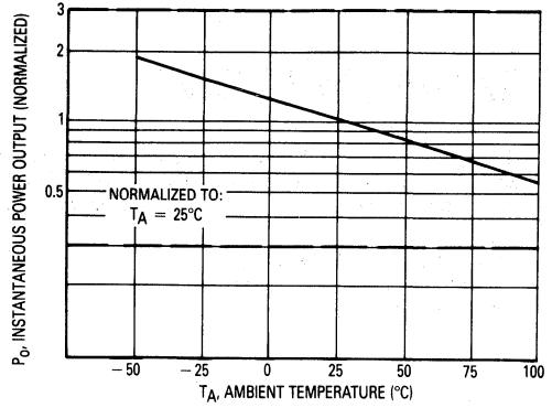
Figure 2. Instantaneous Power Output versus Ambient Temperature
