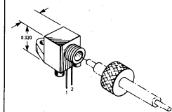
CASE 363B-01 PLASTIC
