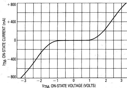
Figure 2. On-State Characteristics
