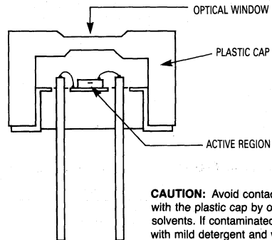
Figure 4. Package Cross Section
