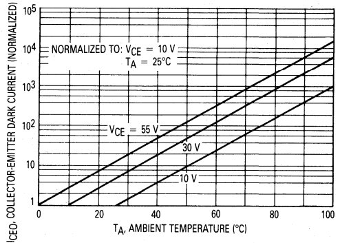
Figure 6. Collector-Emitter Dark Current versus Ambient Temperature
