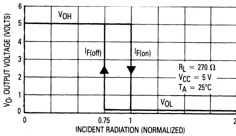
Figure 2. Transfer Characteristics
