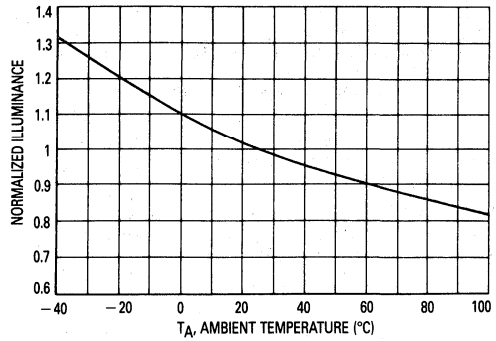
Figure 2. Illuminance versus Temperature
