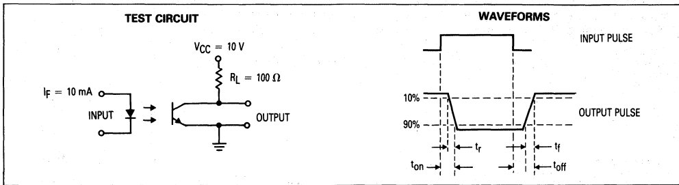
Figure 11. Switching Times
