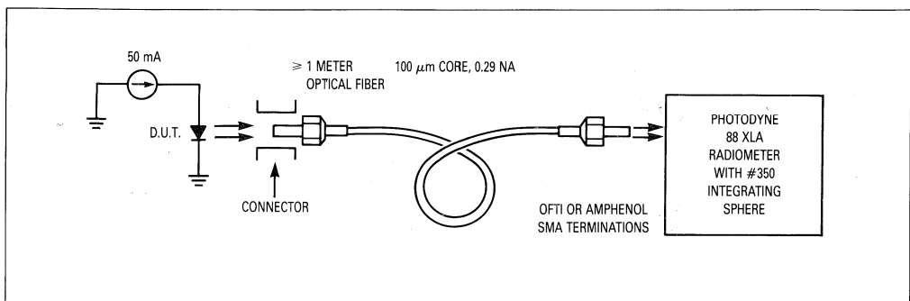
Figure 6. Coupling Efficiency
