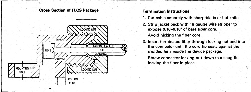
Figure 12. FO Cable Termination and Assembly
