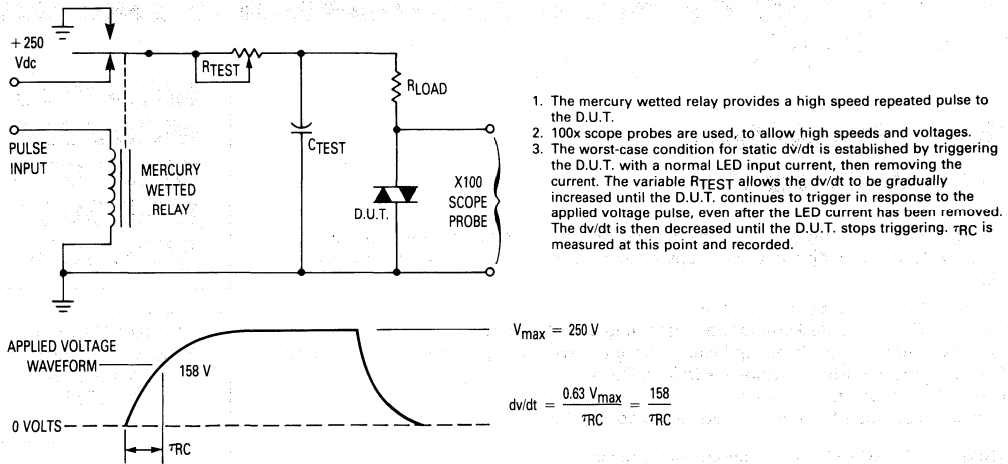
Figure 6. Static dv/dt Test Circuit
