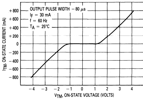
Figure 1. On-State Characteristics
