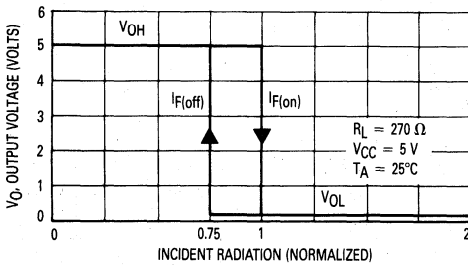
Figure 2. Transfer Characteristics
