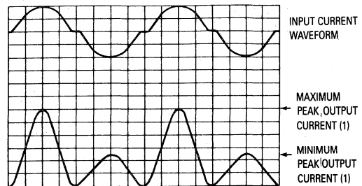
Figure 2. Output Characteristics
