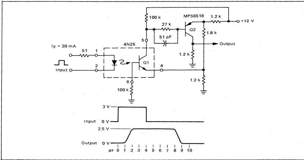
FIGURE 16 – Optically Coupled Schmitt Trigger
