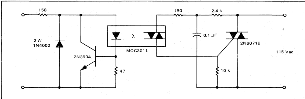
FIGURE 10 – Solid-State Relay
