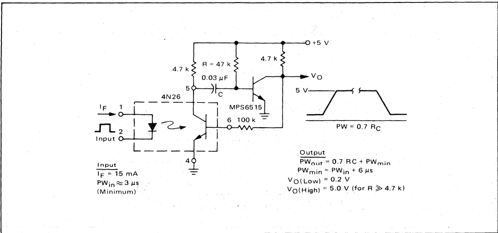
FIGURE 15 – Pulse Stretcher
