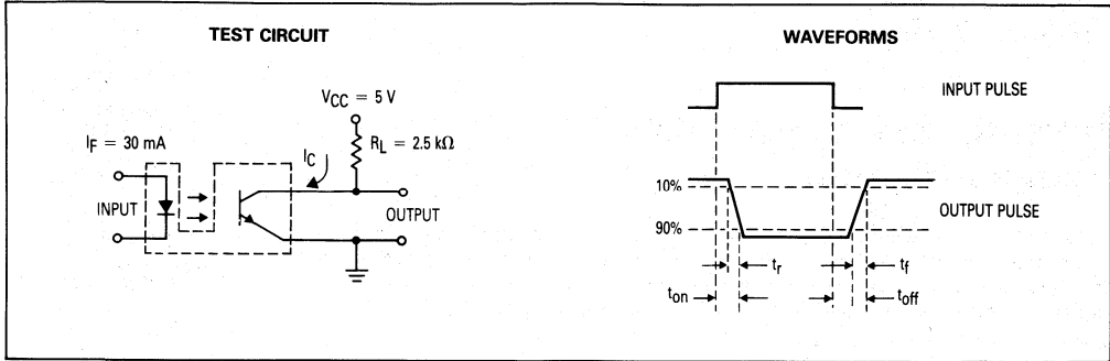
Figure 9. Switching Times
