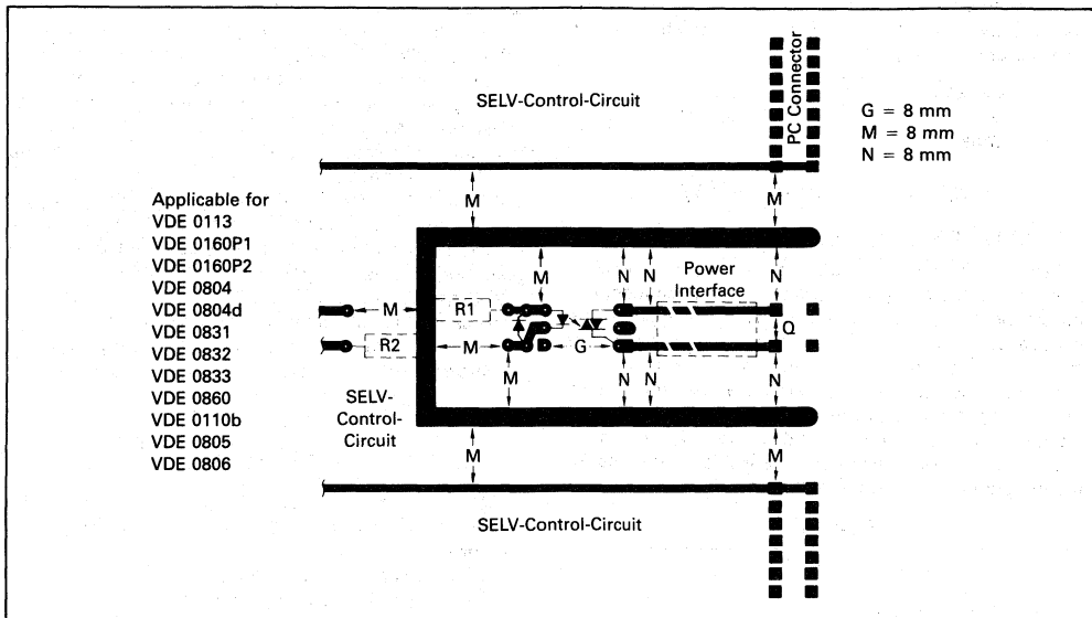
Figure 9. Optocoupler Mounting on PC Board According to Safety Class I with Only One PC Board Plug Connection
