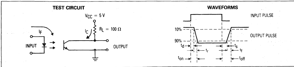
Figure 11. Switching Times
