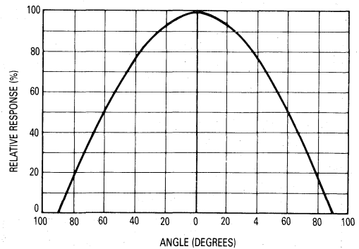
Figure 6. Angular Response
