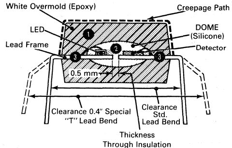
Figure 1. "DOME" Package
