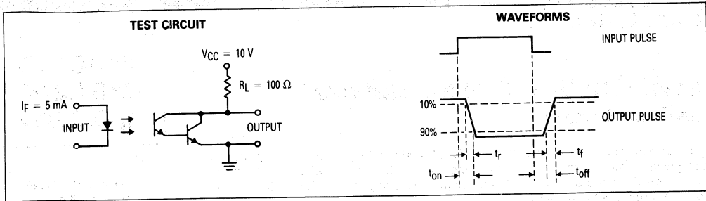
Figure 9. Switching Times
