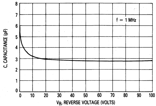
Figure 4. Capacitance versus Voltage
