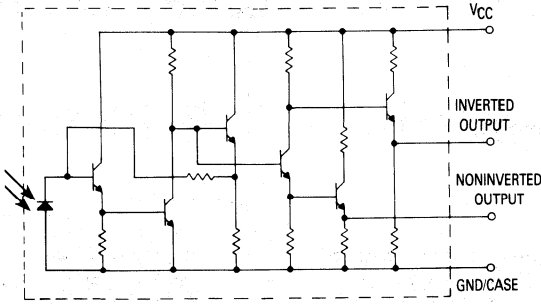
Figure 1. Equivalent Schematic
