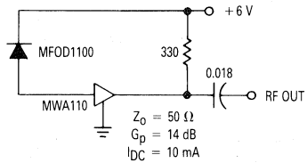
Figure 12. Receiver Circuits
