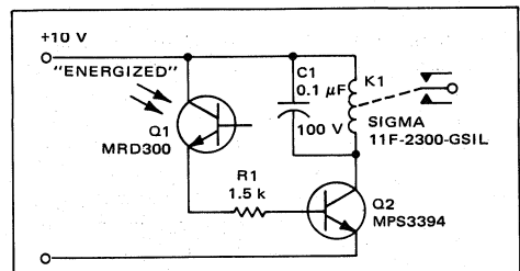
FIGURE 25 – Light-Operated Relay
